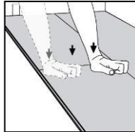
Fig 8b Angle the plank down with a slight press to the left to the short end of the previous plank. Again, using the tapping block tap it against the long end into the previous row. During the fold /angle down, make sure the planks are tight against each other.
