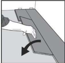
Fig 8b Angle the plank down with a slight press to the left to the short end of the previous plank. Again, using the tapping block tap it against the long end into the previous row. During the fold /angle down, make sure the planks are tight against each other.
