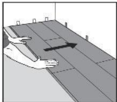
Fig 9. After 2-3 rows. Adjust the distance to the front wall by placing spacer's 12- 15 mm. Once the adjustment is done against the main wall, continue to install till the last row.
