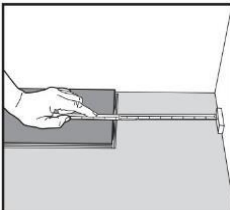
Fig 4. At the end of the first row, put a spacer 12 - 15 mm at the wall and measure the length of the last plank to fit.
